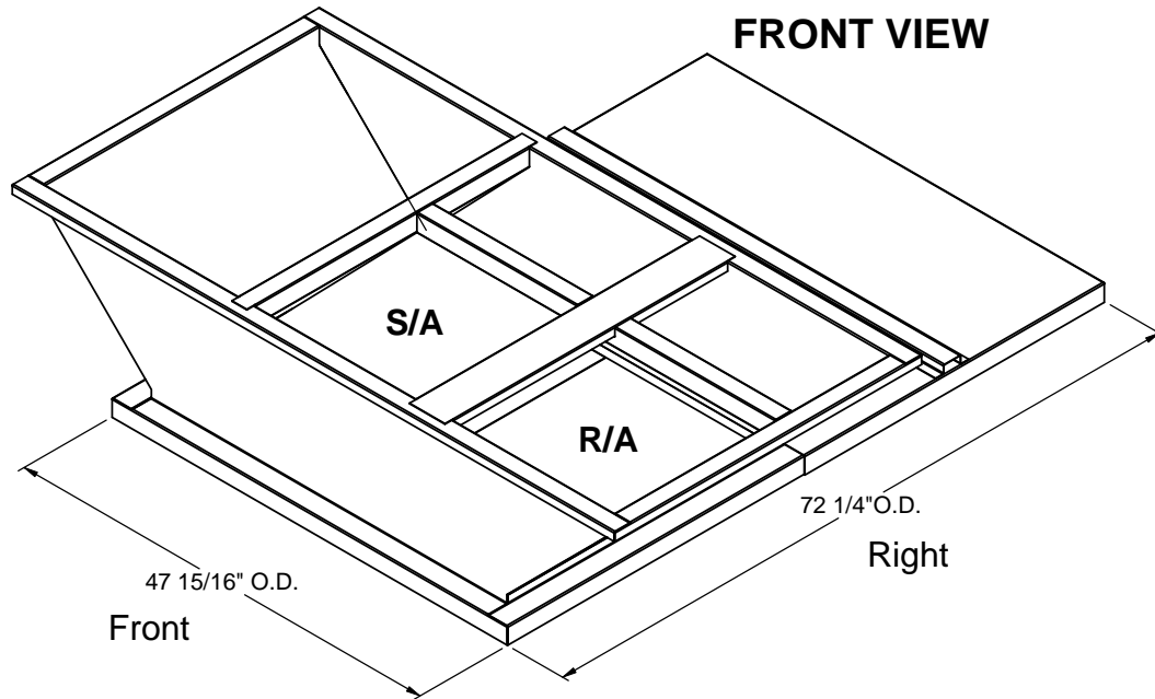
ISOMETRIC VIEW
