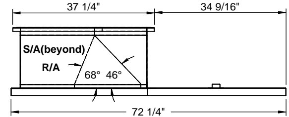
RIGHT VIEW
