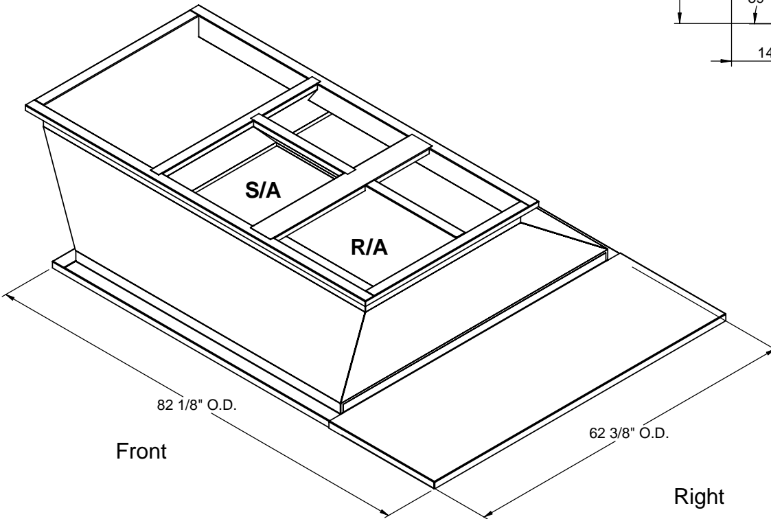
ISOMETRIC VIEW
