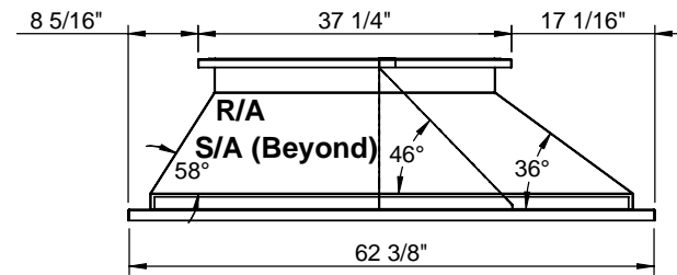
RIGHT VIEW
