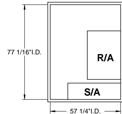
EXISTING CURB
