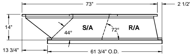
RIGHT VIEW
