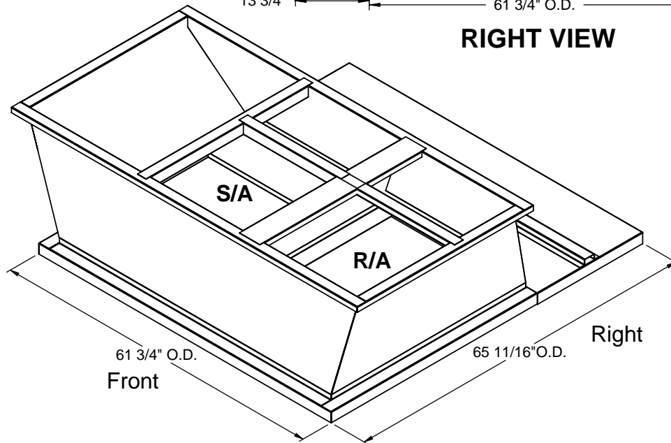
ISOMETRIC VIEW
