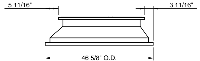
RIGHT VIEW
