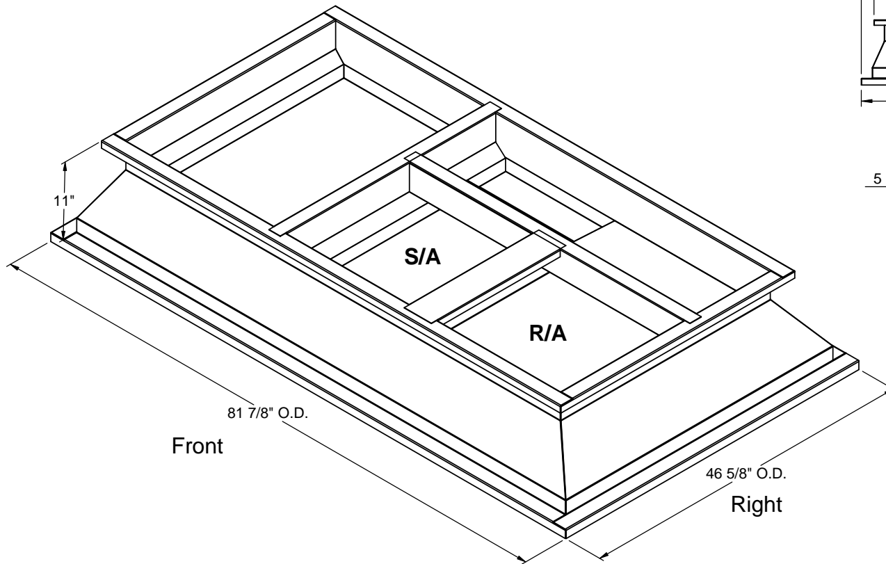
ISOMETRIC VIEW
