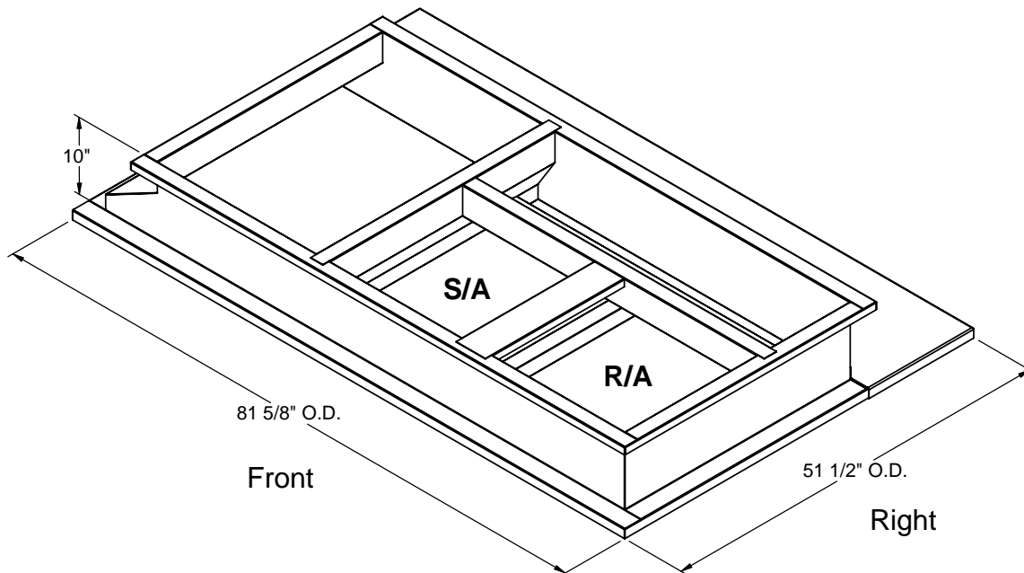
ISOMETRIC VIEW
