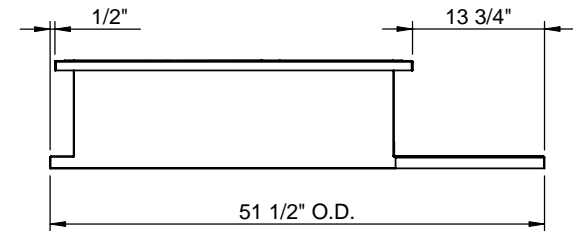
RIGHT VIEW
