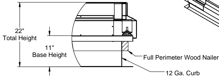
SIDE VIEW DETAIL
