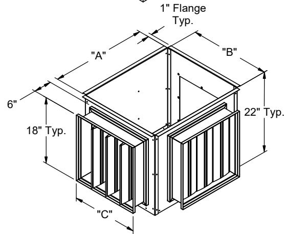
Example Shown P/N: MB-ADP-AX3060**-FA
