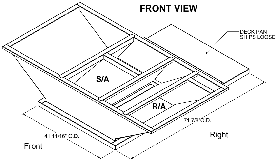
ISOMETRIC VIEW
