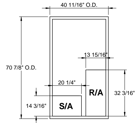
EXISTING CURB
