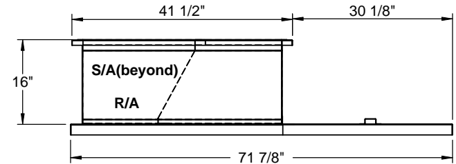
RIGHT VIEW
