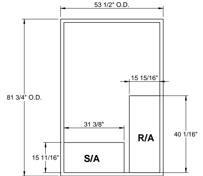
EXISTING CURB
