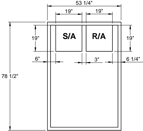
EXISTING CURB
