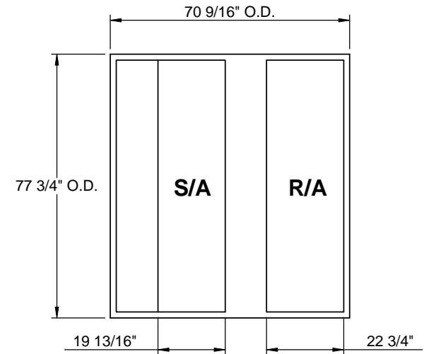
EXISTING CURB
