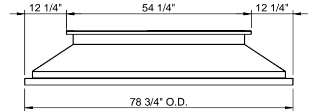
RIGHT VIEW
