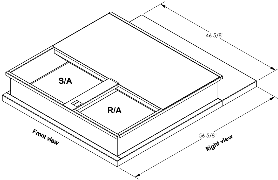
ISOMETRIC VIEW
