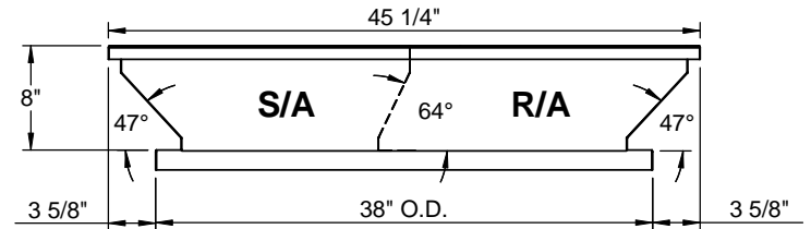
RIGHT VIEW
