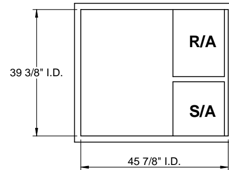
EXISTING CURB
