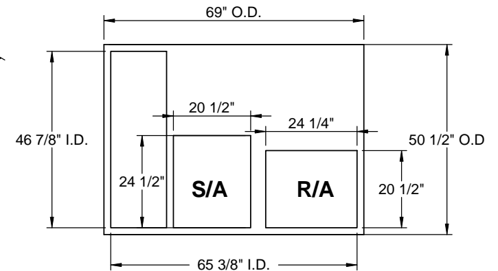
EXISTING CURB
