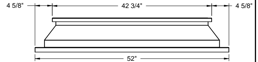
RIGHT VIEW
