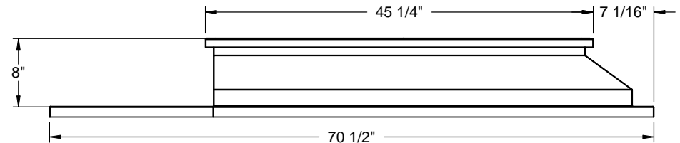
FRONT VIEW
