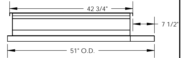
RIGHT VIEW
