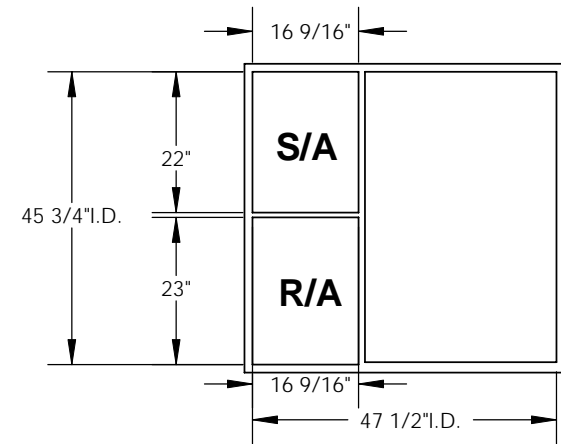
EXISTING CURB
