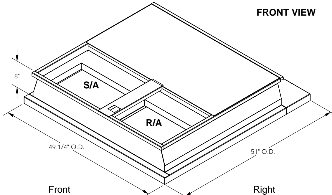
ISOMETRIC VIEW
