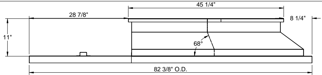
FRONT VIEW
