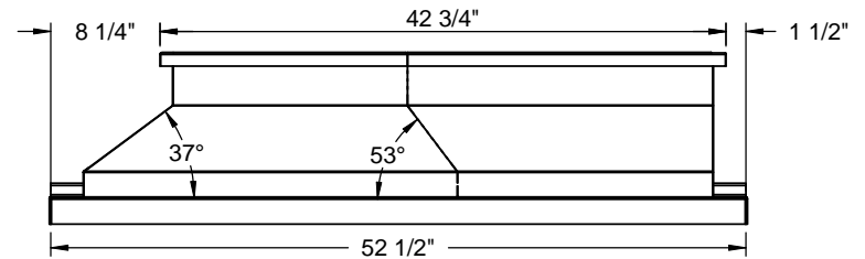
RIGHT VIEW
