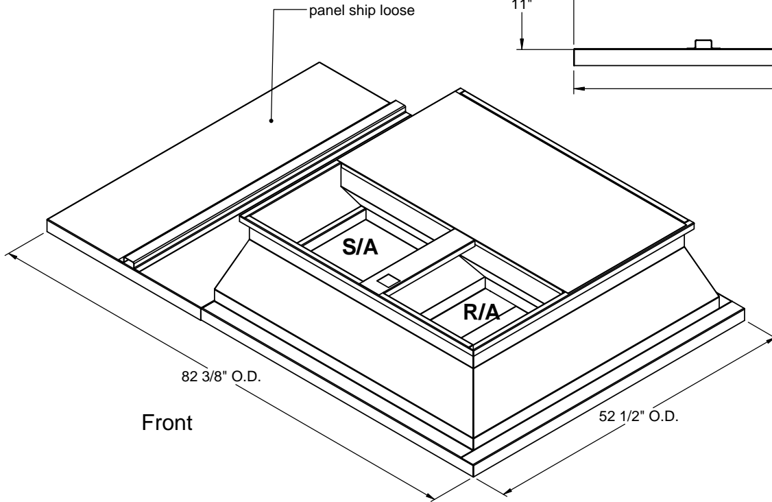
ISOMETRIC VIEW
