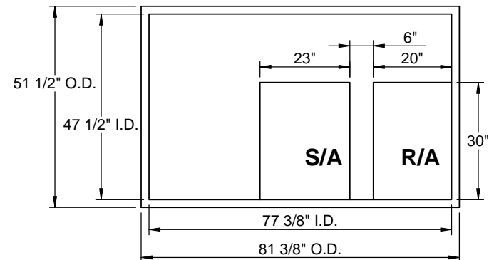
EXISTING CURB
