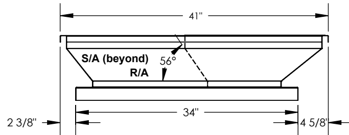
RIGHT VIEW
