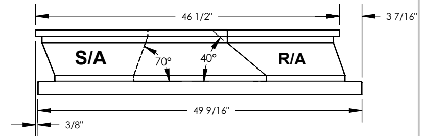
FRONT VIEW
