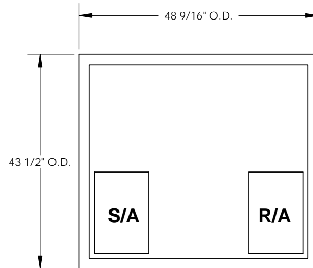
EXISTING CURB
