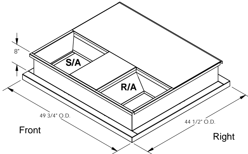
ISOMETRIC VIEW
