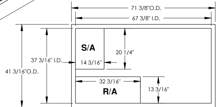
EXISTING CURB
