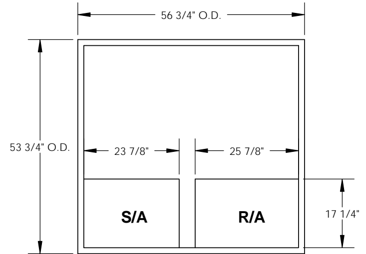
RIGHT VIEW
