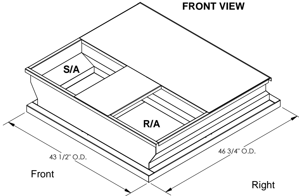
ISOMETRIC VIEW
