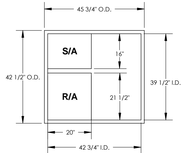
EXISTING CURB
