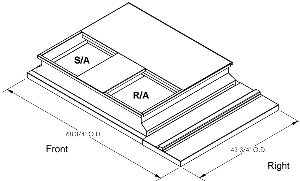
ISOMETRIC VIEW
