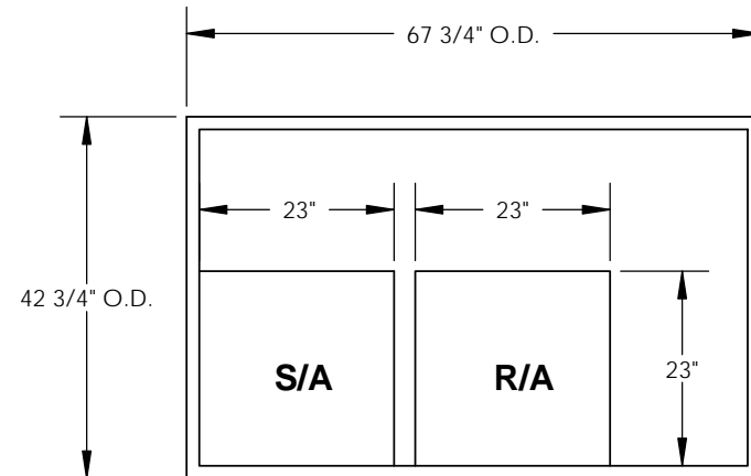
EXISTING CURB
