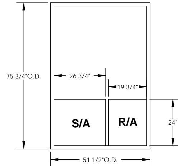
EXISTING CURB
