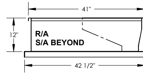
RIGHT VIEW
