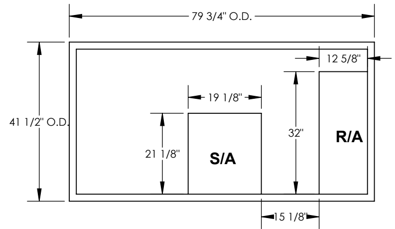
EXISTING CURB
