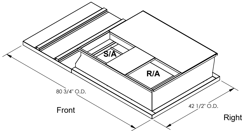
ISOMETRIC VIEW
