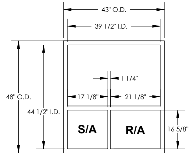
EXISTING CURB
