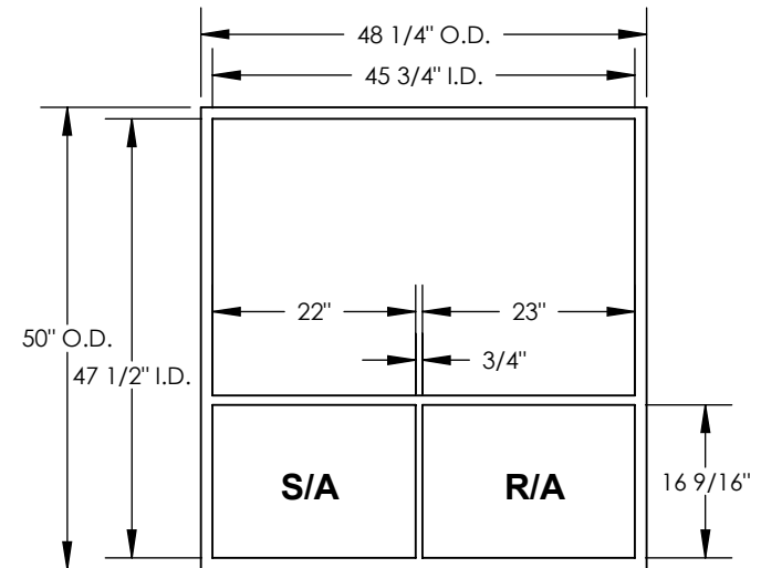
EXISTING CURB
