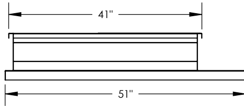
RIGHT VIEW
