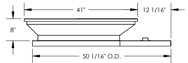
RIGHT VIEW
