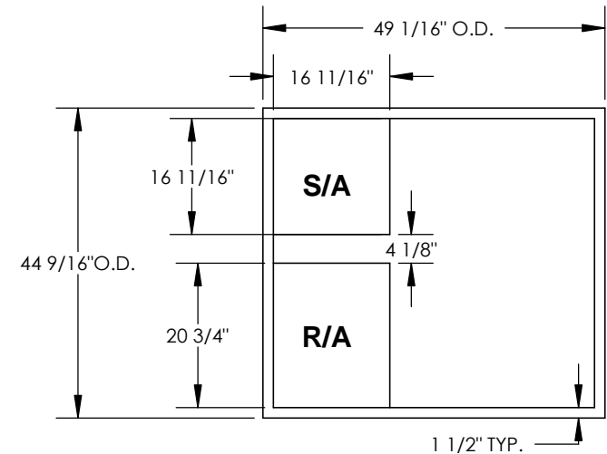
EXISTING CURB
