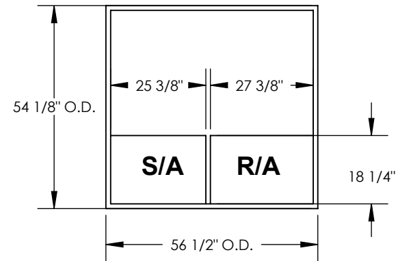
EXISTING CURB
