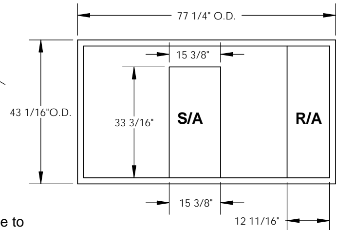
EXISTING CURB
