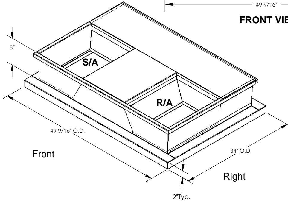
ISOMETRIC VIEW
