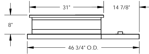
RIGHT VIEW
