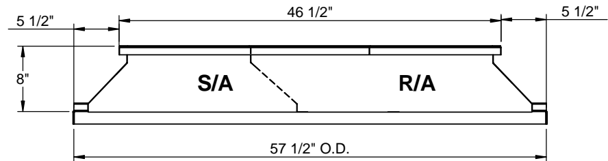
RIGHT VIEW
