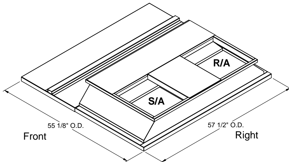
ISOMETRIC VIEW
