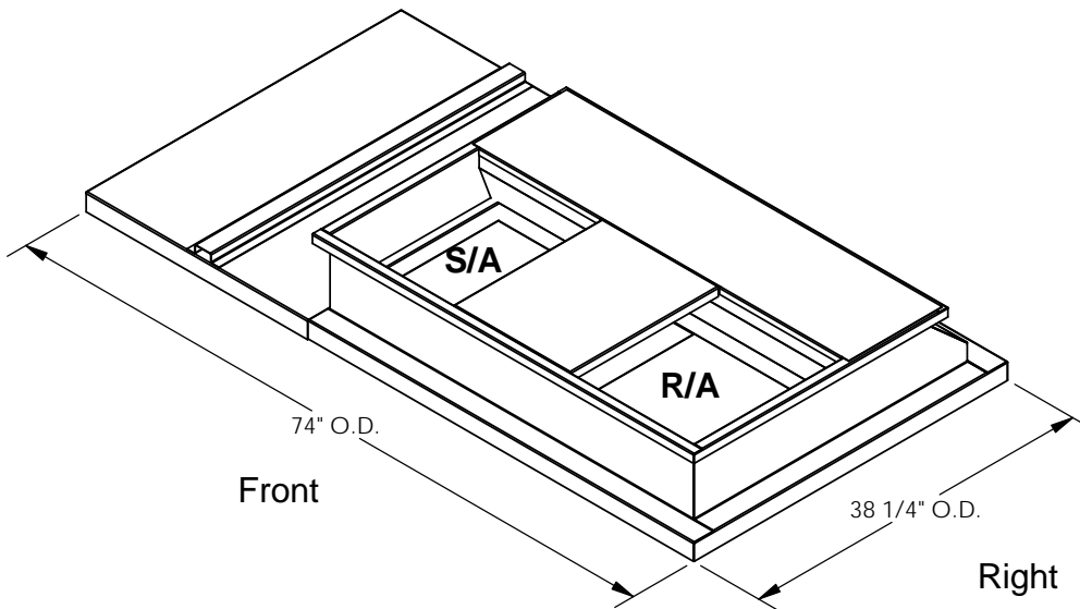
ISOMETRIC VIEW
