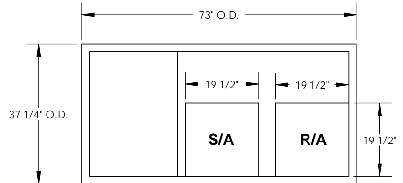
EXISTING CURB
