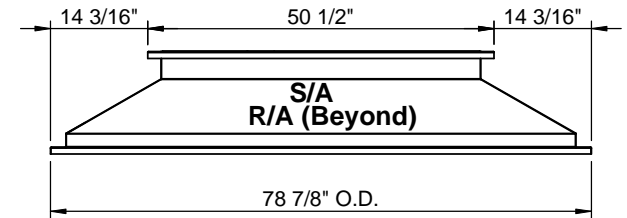
RIGHT VIEW
