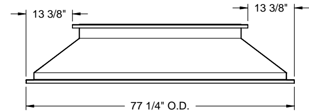
RIGHT VIEW
