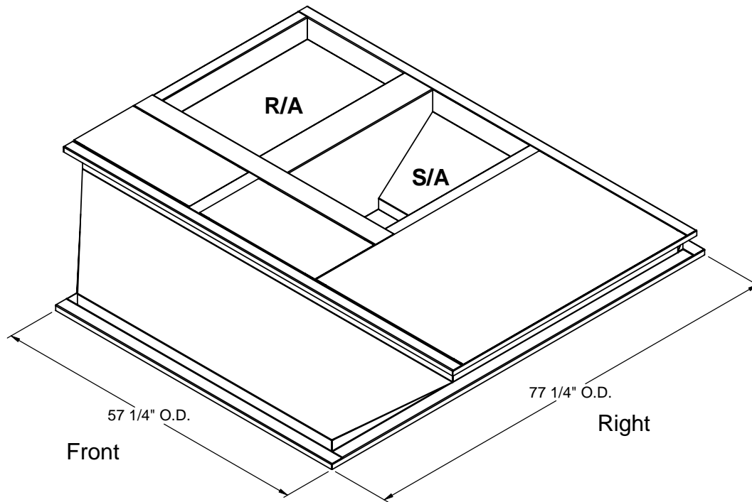
ISOMETRIC VIEW
