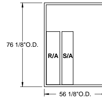
EXISTING CURB
