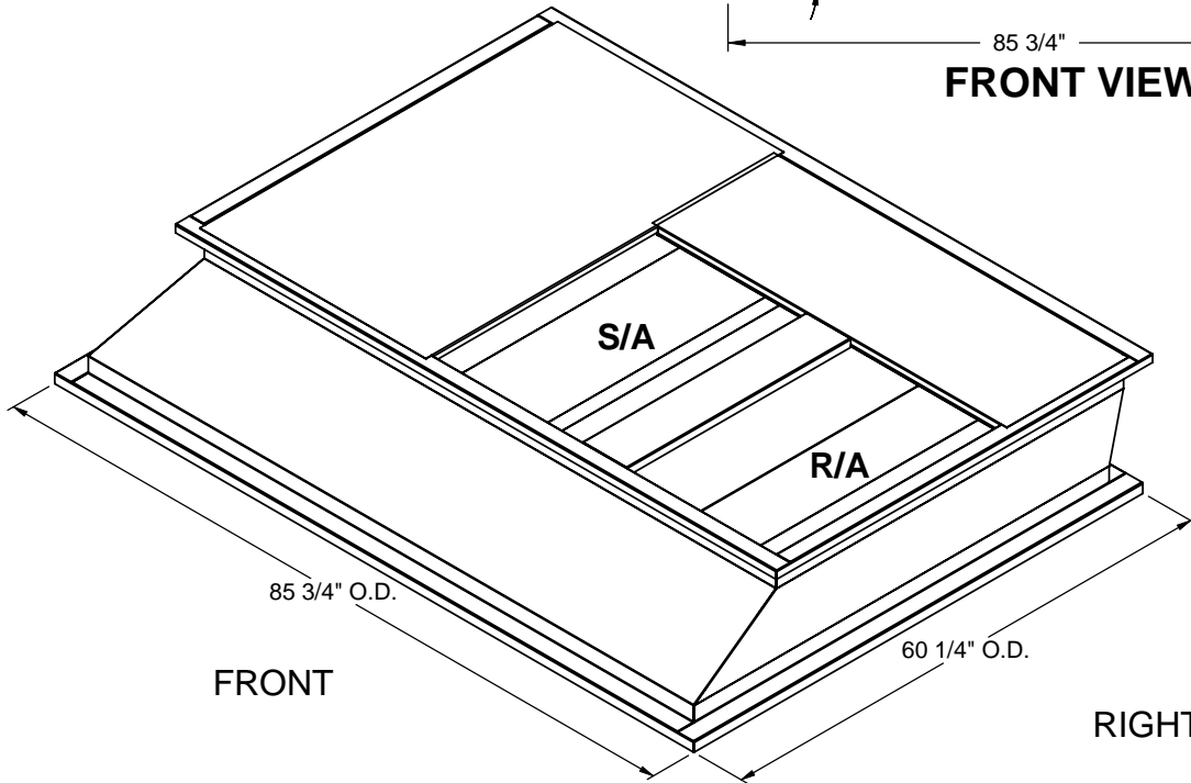
ISOMETRIC VIEW
