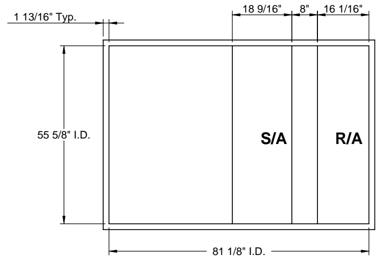
EXISTING CURB
