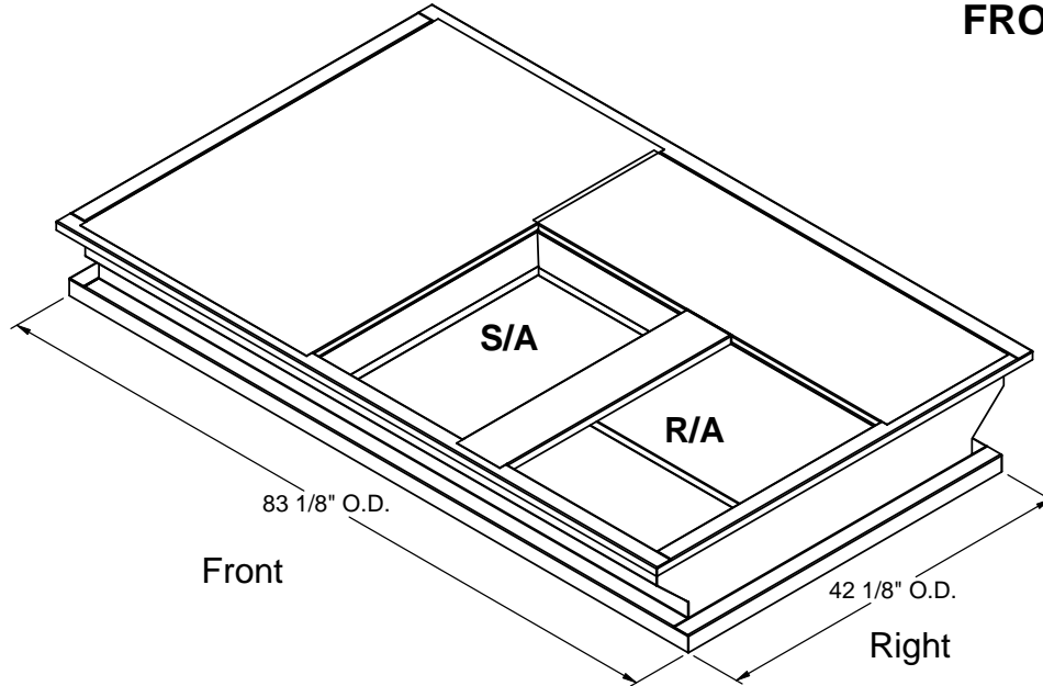
ISOMETRIC VIEW
