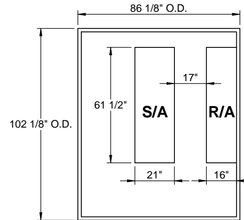
EXISTING CURB
