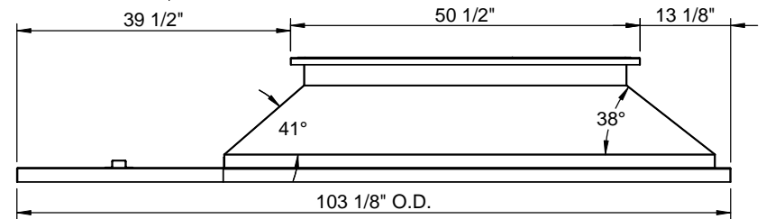
RIGHT VIEW
