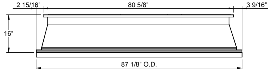
FRONT VIEW
