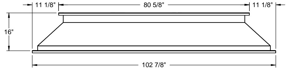
FRONT VIEW
