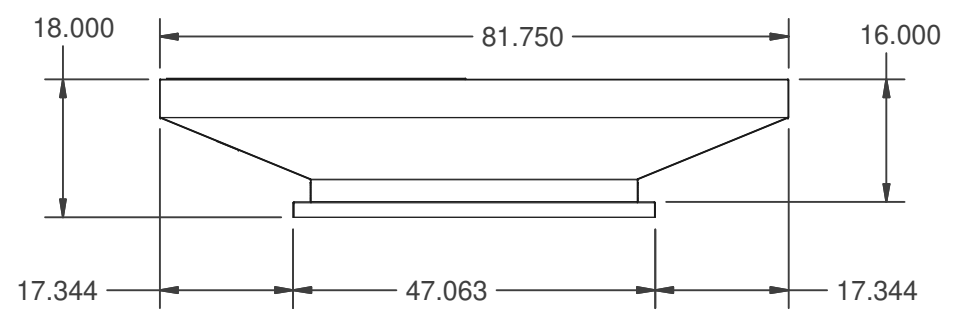
SIDE VIEW
