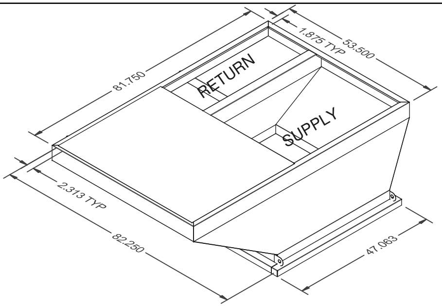
ISO VIEW
