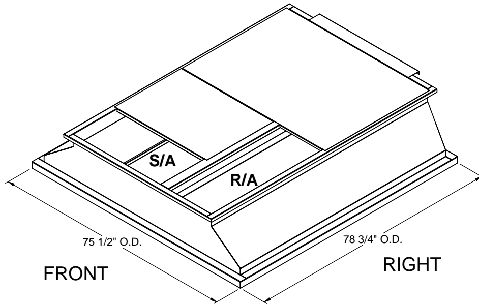
ISOMETRIC VIEW
