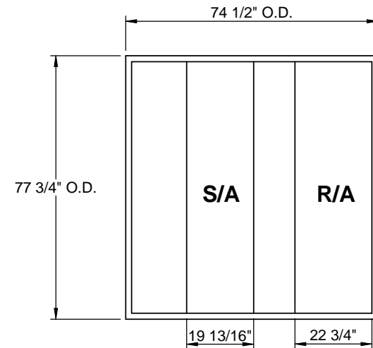
EXISTING CURB
