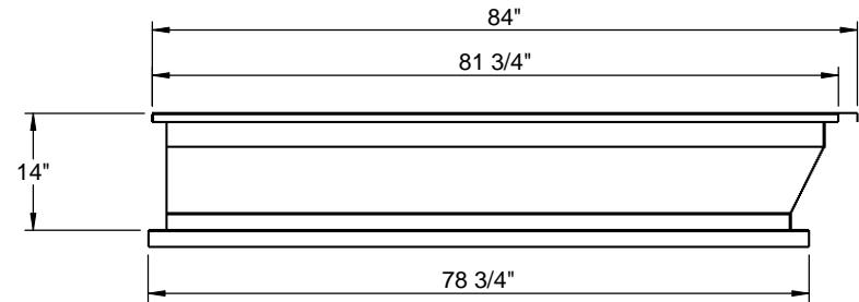
RIGHT VIEW
