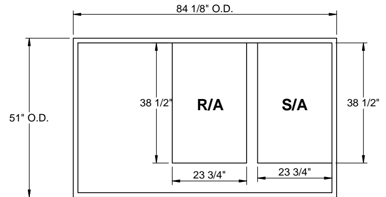
EXISTING CURB
