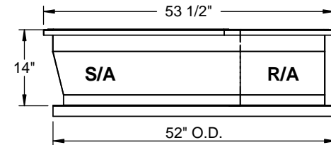
RIGHT VIEW
