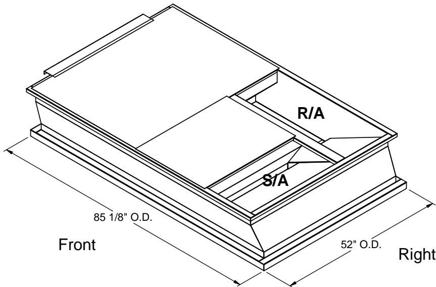
ISOMETRIC VIEW
