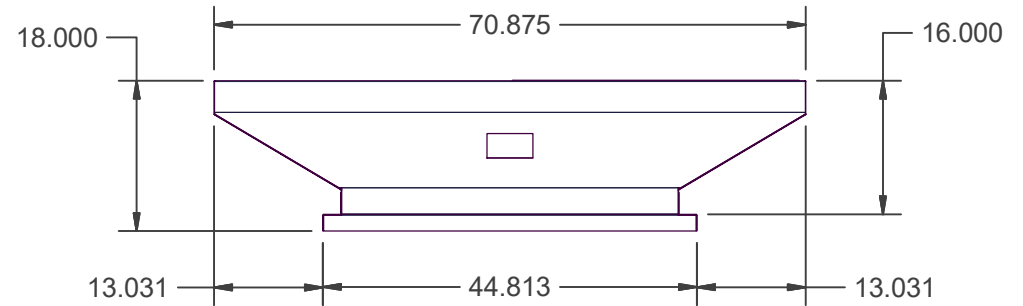
FRONT VIEW
