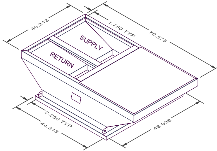
ISO VIEW
