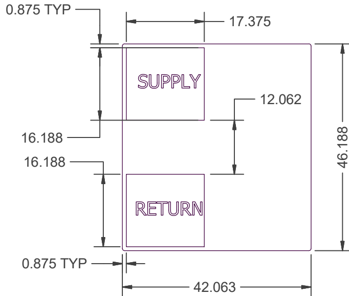
EXISTING CURB
