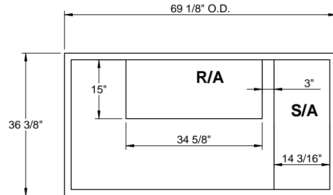
EXISTING CURB
