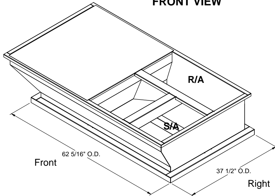
ISOMETRIC VIEW
