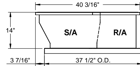
RIGHT VIEW
