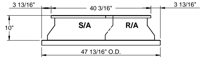
RIGHT VIEW
