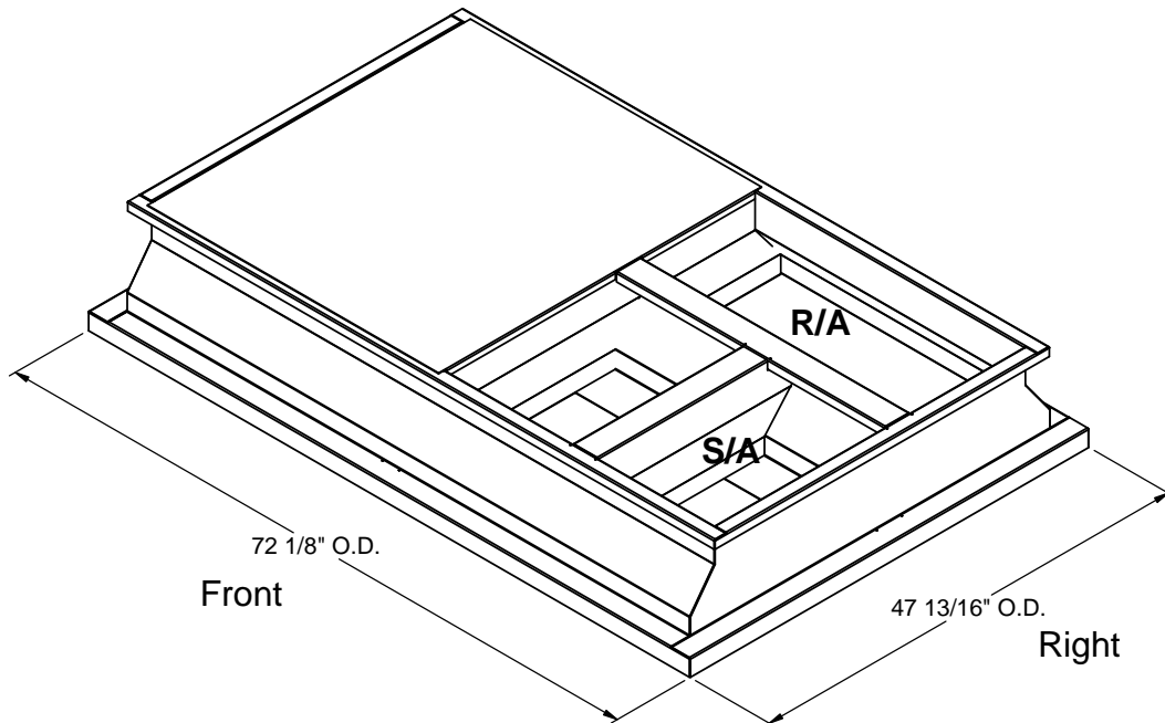
ISOMETRIC VIEW
