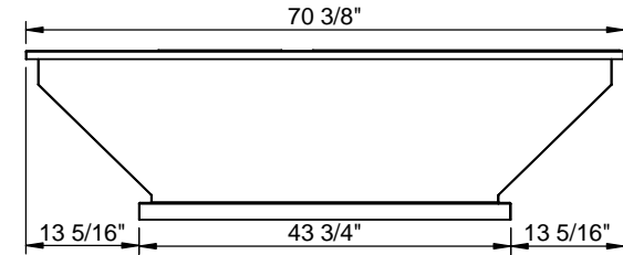
RIGHT VIEW
