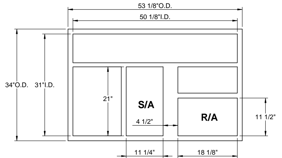
EXISTING CURB
