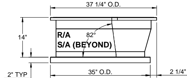
RIGHT VIEW
